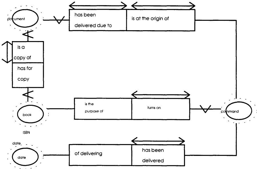
Figure 6.2: Example of NIAM Schema.
