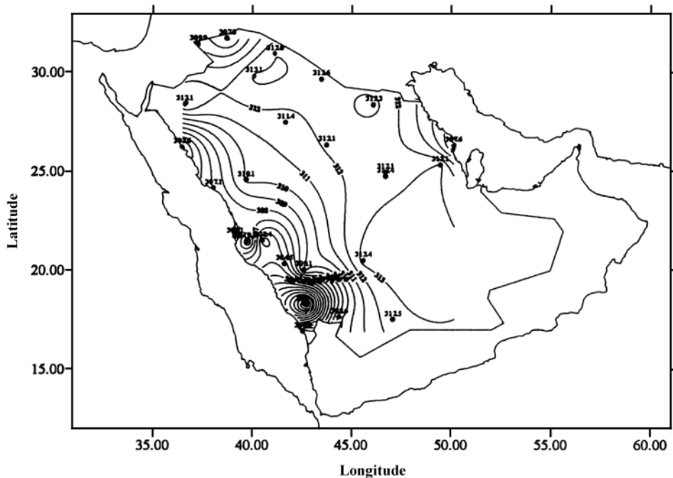
FIG. 1. Isothermal map ( ^{\circ}\text{K} ) of study area for September 08, 1987, at 15 GMT.
