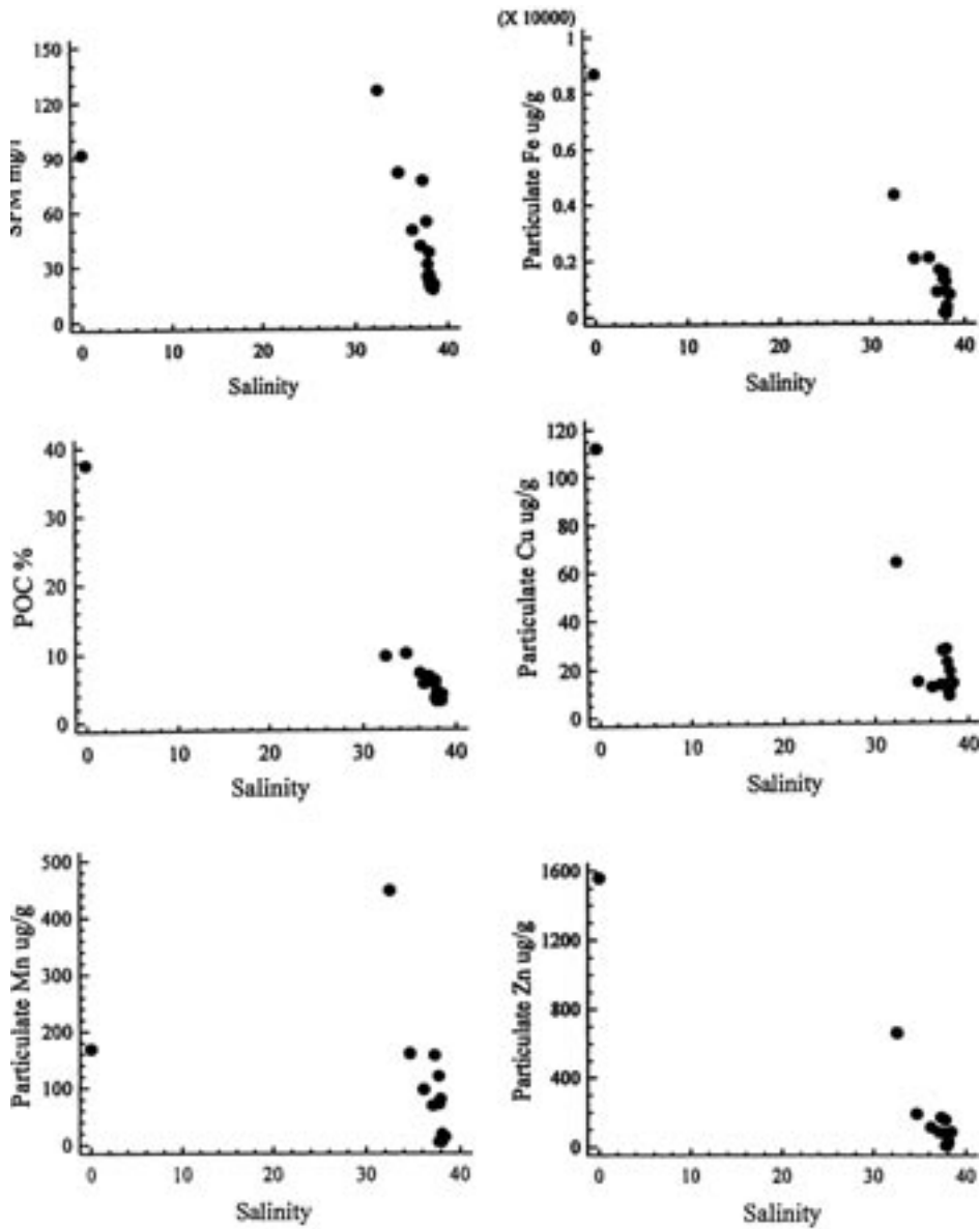
FIG. 7. Relationship between salinity and SPM, POC, particulate Mn, Fe, Cu and Zn in the dilution basin.
