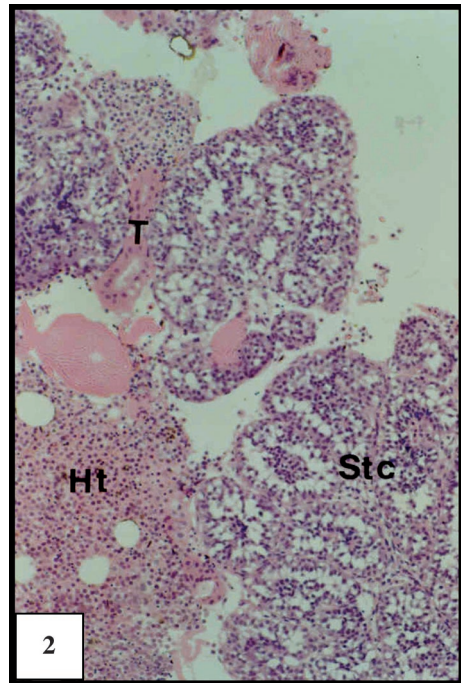
Fig. 1. Light micrograph of Stannius corpuscles (Stc) of large tilapia showing embedding of highly lobulated Stc in the trunk kidney. (BV) large blood vessel, (T) kidney tubules. H&E \times 320.
