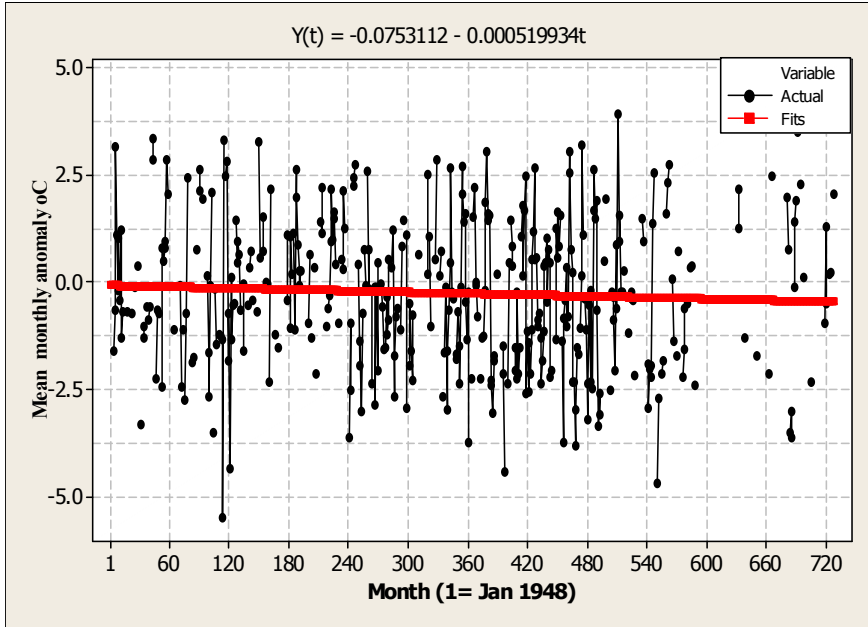
Fig. 2a. Linear trend analysis plot for mean monthly SSTA.
