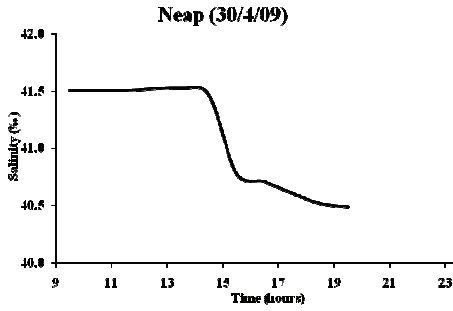
Fig. 10. Salinity variation over a tidal cycle on the 30 th April 2009 at neap tide.
