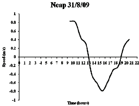
Fig. 22. Current velocity variations over a tidal cycle on the 31 st August 2009 at neap tide.
