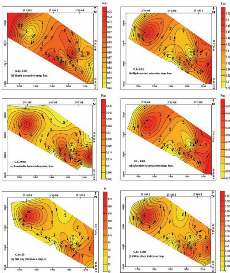
Fig. 8. Reservoir fluid distribution maps of Bahariya Formation in Meleiha-NE oil field, north Western Desert, Egypt.
