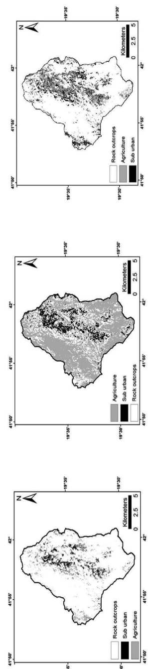
Fig. 5. Supervised classification methods applied to Wadi Al Hamid.
