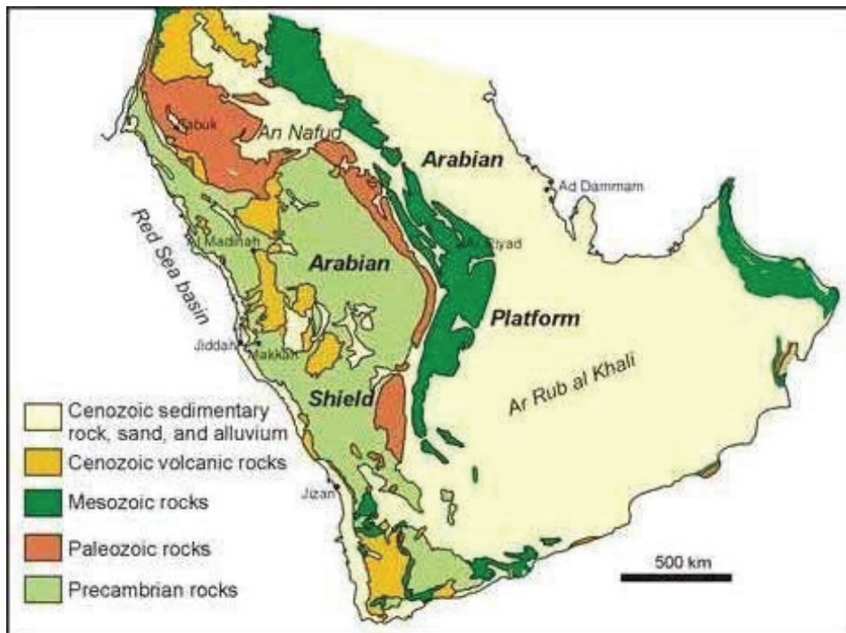
Fig. 1. Arabian Peninsula and the Arabian Shelf.
