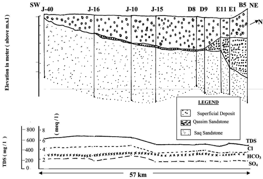
Fig. 4. SW-NE geologic cross-section and a hydrochemical profile along the study area.
