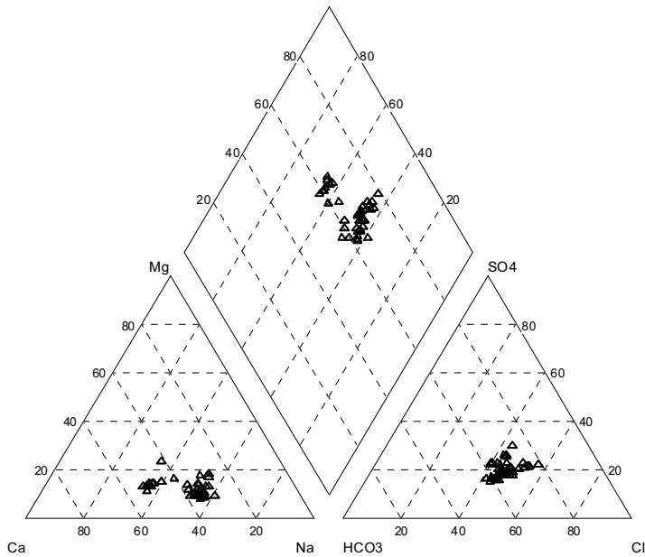
Fig. 5. Piper's diagram showing the general hydrochemical characteristics of the Saq aquifer.
