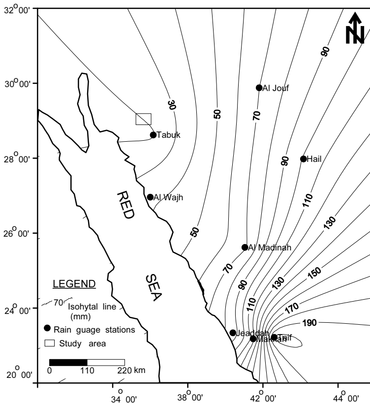
Fig. 2. Location map of the study area and the average annual rainfall.
