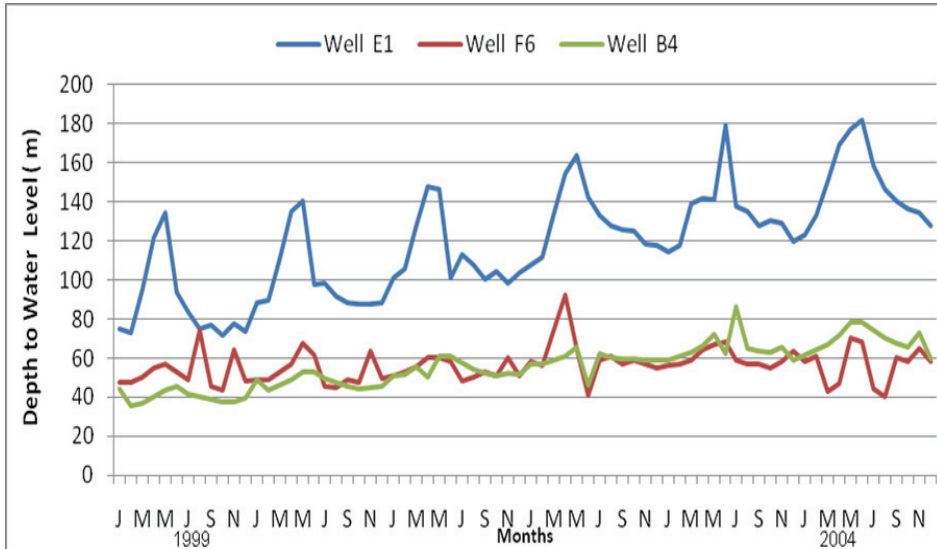
Fig. 6. Annual fluctuation of water levels in selected wells during the period 1999-2004.
