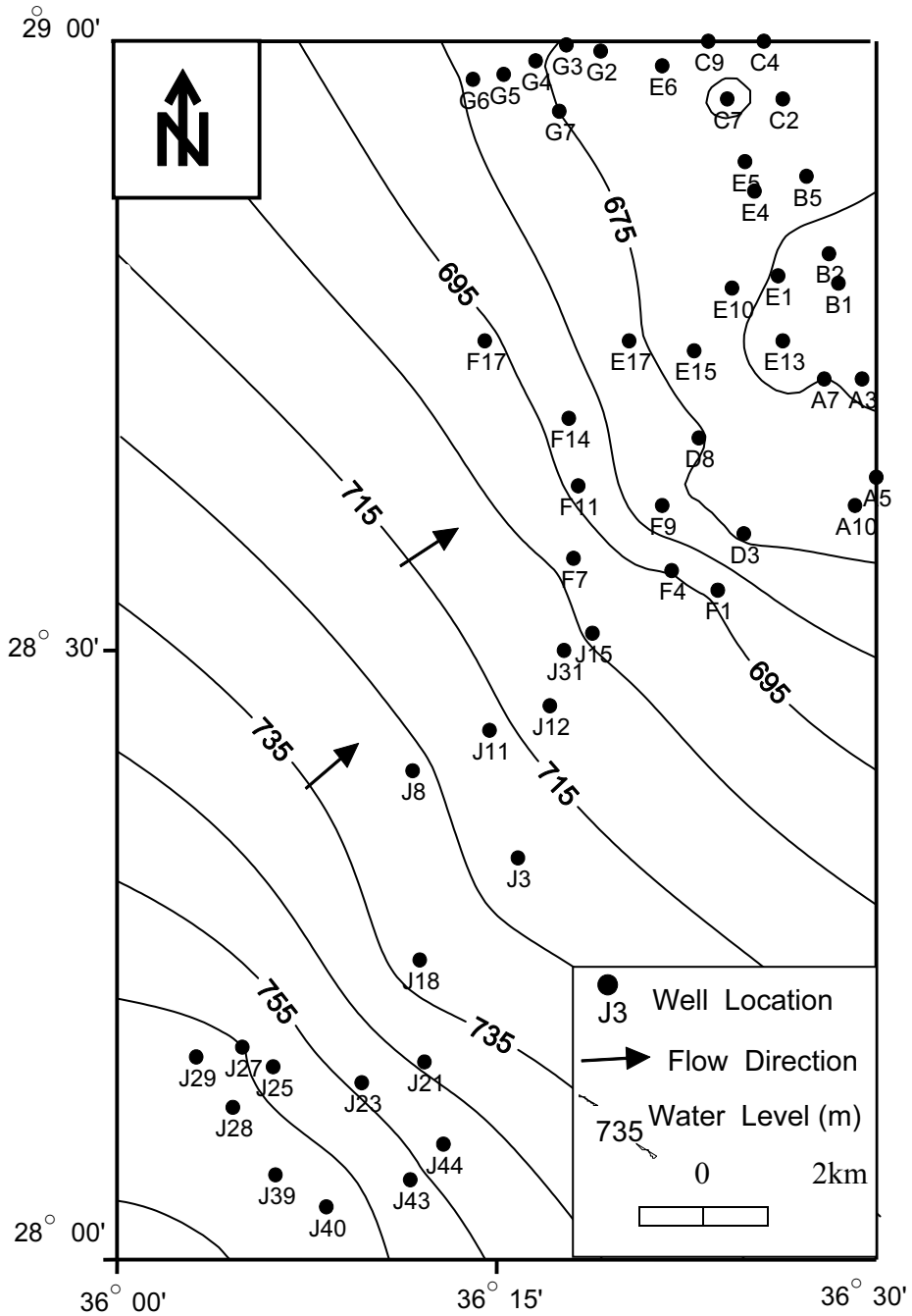
Fig. 3. Water level contour map of the study area in 2004.
