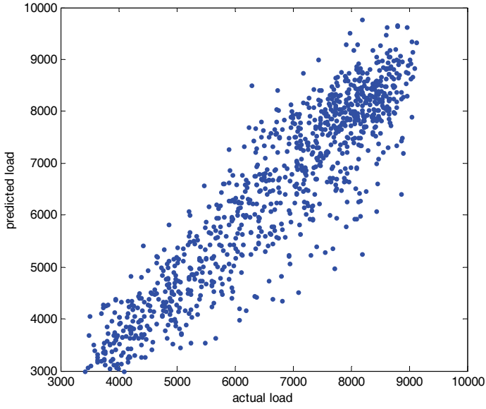
Fig. 11. NN committee machine predicted against actual load for testing data.
