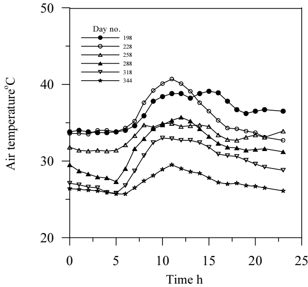
Fig. 3 (b). Dry bulb temperature variation for the city of Jeddah, KSA for 6 months.
