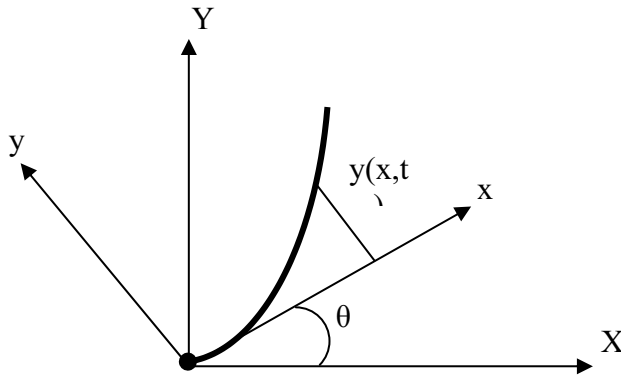
Fig. 1. Rotating flexible beam model.
