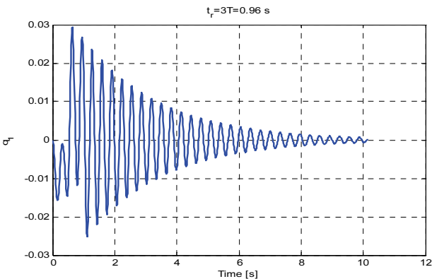
Fig. 3. Rotating beam vibration for t_r=3T .
