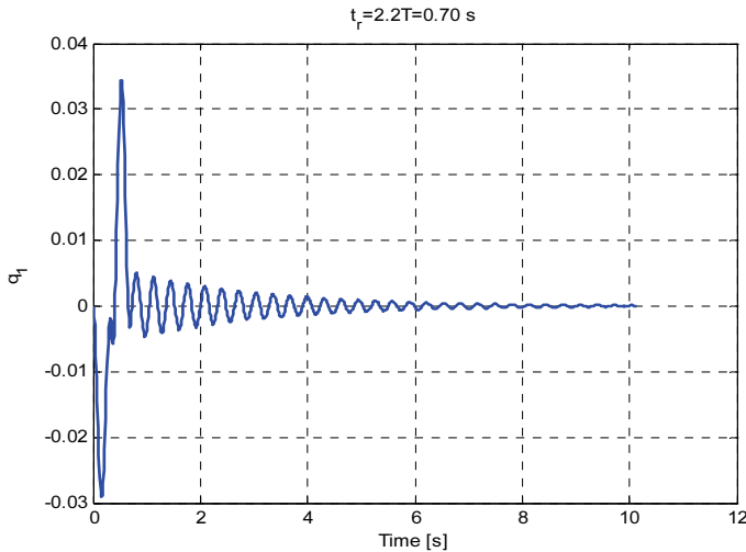
Fig. 2. Rotating beam vibration for t_r = 2.2T .
