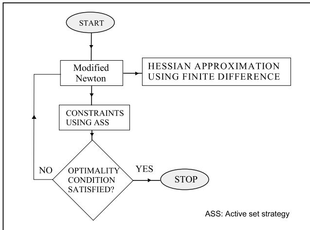
FIG. 2. Structure of the proposed hybrid algorithm.
