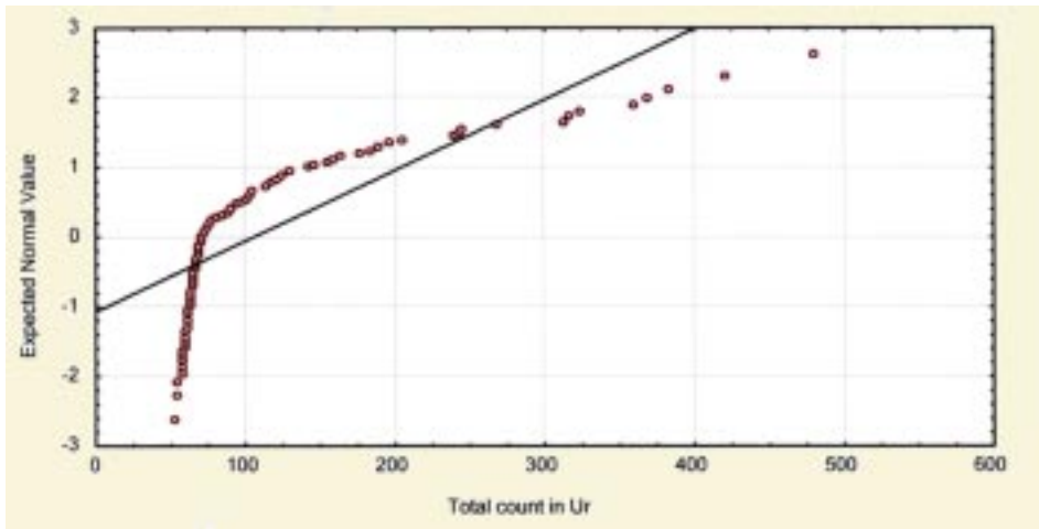
FIG. 16. Normal probability plots of total count radiometric data for AN, Drift II, El-Ereidiya mine, Central Eastern Desert.
