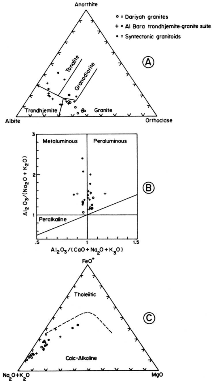
Fig. 3(A-C). (A) Normative An-Ab-Or diagram (after Barker 1979). (B) Plot of the molecular ratio of A/NK versus A/CNK (A = Al_2O_3 , N = Na_2O , K = K_2O , C = CaO ). (C) AFM diagram showing calc-alkaline trend for all granite groups.
