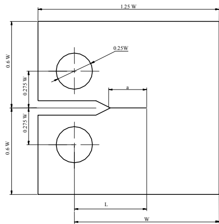
Fig.1. Configuration of compact tension specimen for fatigue and fracture mechanics-based testing.
