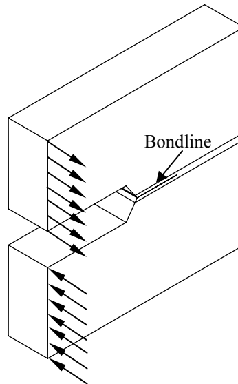
Fig. 6. The out of plane pressure applied to simulate the tear mode.
