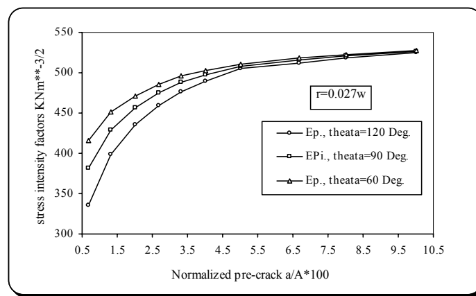
Fig. 9. Effect of the pre-crack length on the stress intensity factor, K_I , for a filler material (Epoxy) for different crack notch angles and r/w = 0.027 .
