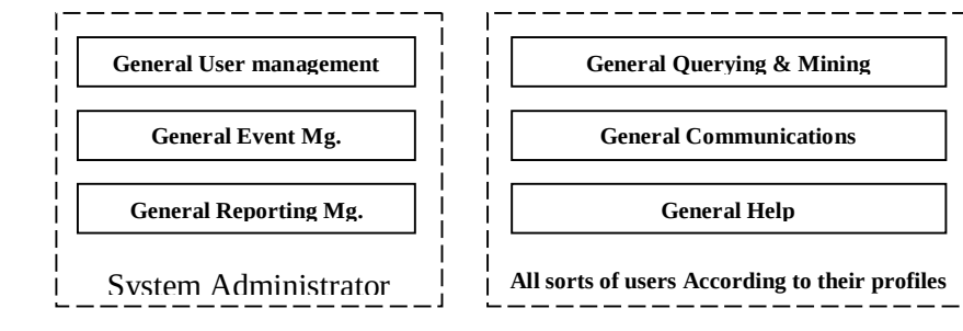
Fig. 6. Management Subsystem.
