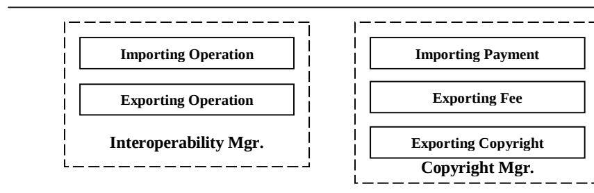
Fig. 7. Community Subsystem.
