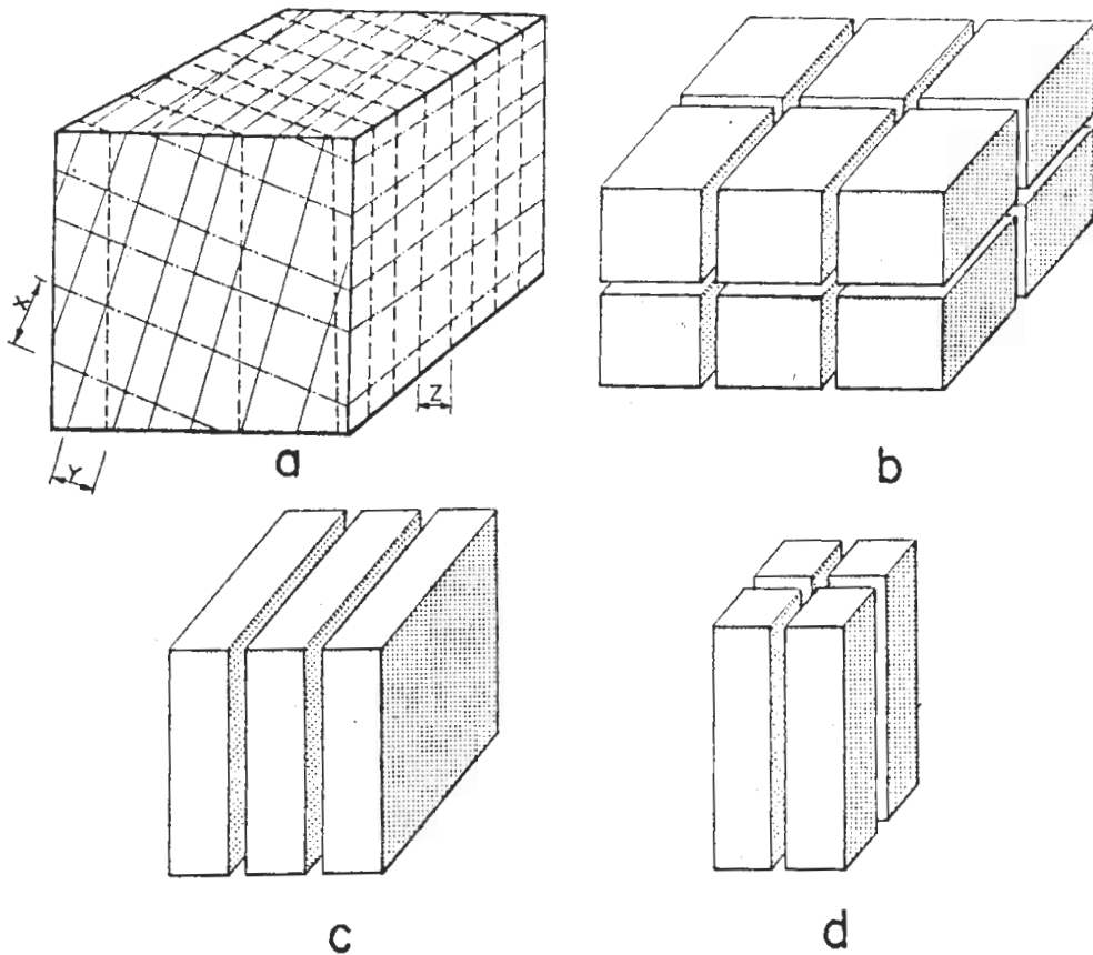
FIG. 1. (a) Block diagram with 3 orthogonal joint sets; (b) Prismatic blocks; (c) plate blocks; (d) bar blocks.
