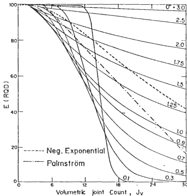
FIG. 9. Plate block RQD-J_v charts, ( \alpha = 0.5 , t = 0.10m ).
