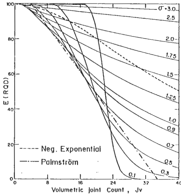
FIG. 18. Prismatic block RQD-J_v charts, ( \alpha = 0.9 , \beta = 0.5 , t = 0.10 m).
