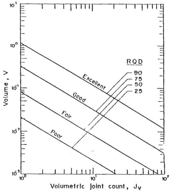
FIG. 20. Prismatic block RQD-J_v-V charts, ( \alpha = 0.5 , \beta = 0.9 , t = 0.10 m).
