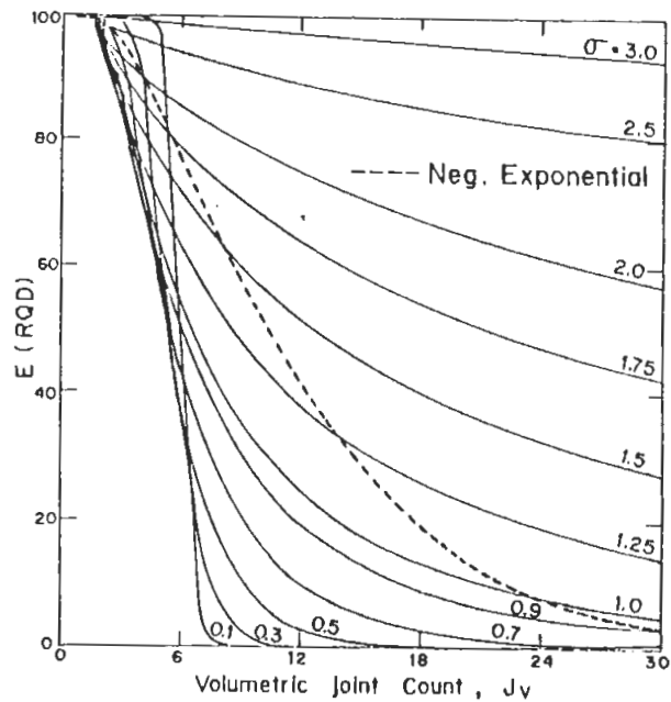
FIG. 8. Plate block RQD-J_v charts, ( \alpha = 0.1 , t = 0.20\text{m} ).
