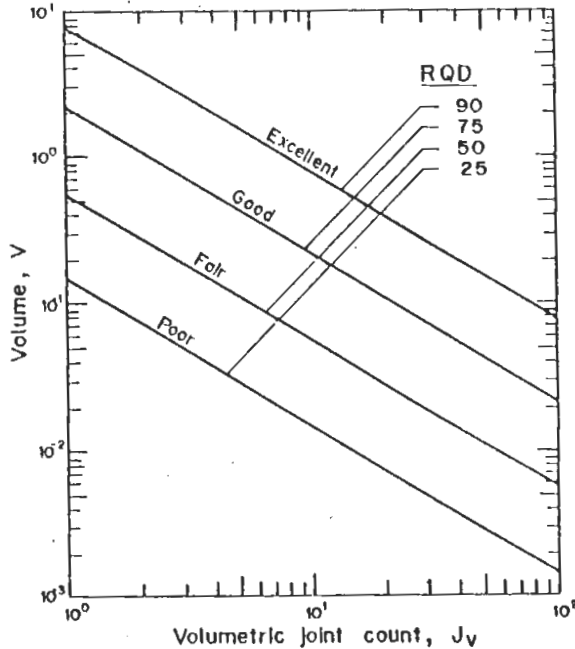
FIG. 21. Prismatic block RQD-J_v-V charts, ( \alpha = 0.9 , \beta = 0.9 , t = 0.10 m).
