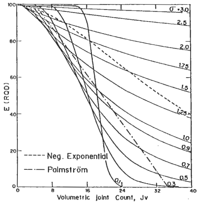
FIG. 17. Prismatic block RQD-J_v charts, ( \alpha = 0.5 , \beta = 0.5 , t = 0.10 m).
