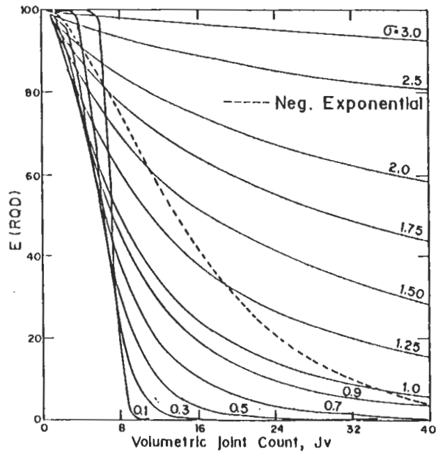
FIG. 16. Prismatic block RQD-J_v charts, ( \alpha = 0.1 , \beta = 0.5 , t = 0.20 m).
