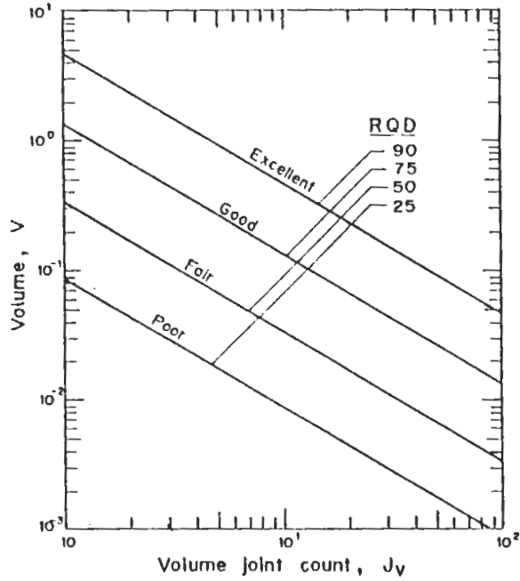
FIG. 19. Prismatic block RQD-J_v-V charts, ( \alpha = 0.1 , \beta = 0.5 , t = 0.10 m).
