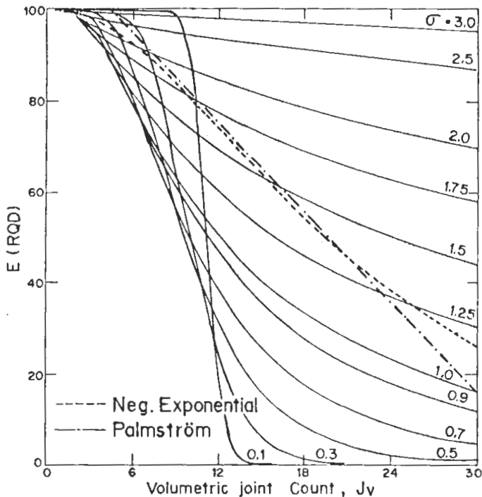
FIG. 6. Plate block RQD-J_v charts, ( \alpha = 0.1 , t = 0.10m ).
