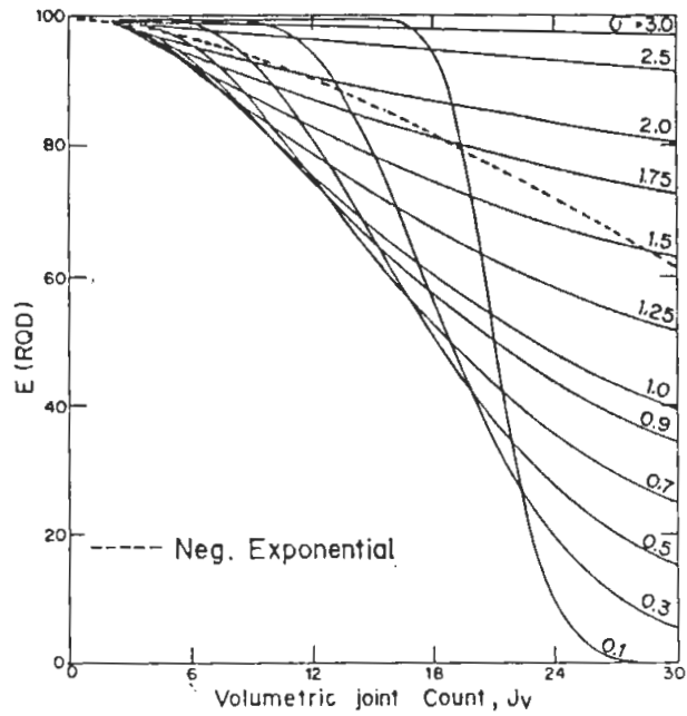
FIG. 7. Plate block RQD-J_v charts, ( \alpha = 0.1 , t = 0.05\text{m} ).
