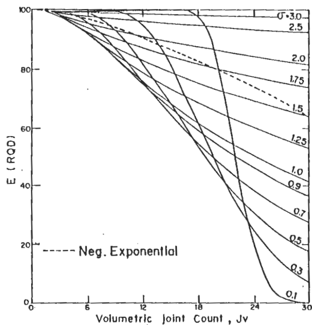
FIG. 15. Prismatic block RQD-J_v charts, ( \alpha = 0.1 , \beta = 0.5 , t = 0.05 m).
