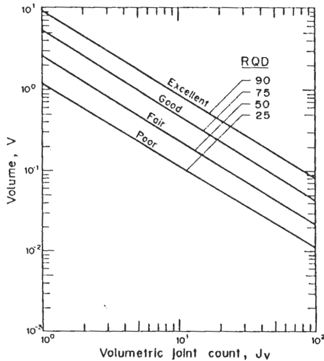
FIG. 13. Plate block RQD-J_v-V charts. ( \alpha = 0.9 ).
