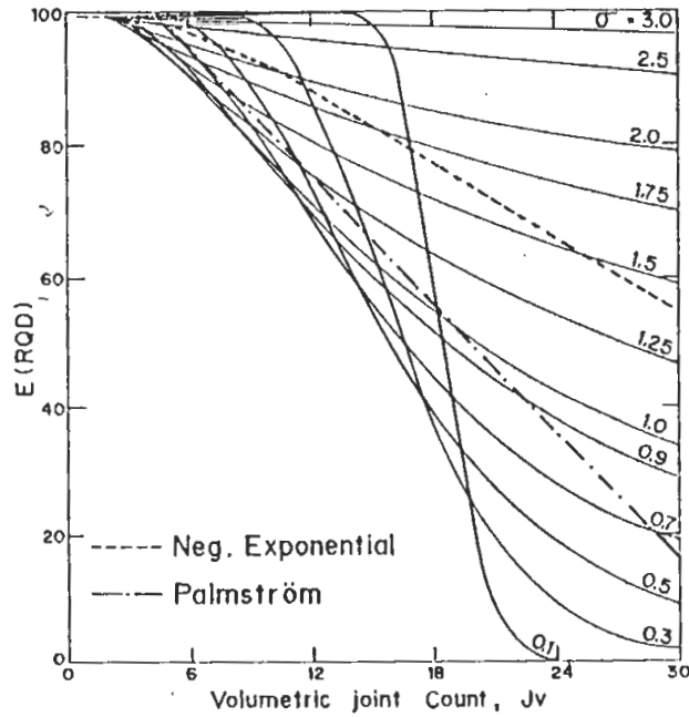
FIG. 10. Plate block RQD-J_v charts, ( \alpha = 0.9, t = 0.10m ).
