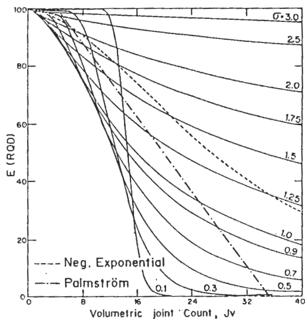
FIG. 14. Prismatic block RQD-J_v charts, ( \alpha = 0.1 , \beta = 0.5 , t = 0.10 m).
