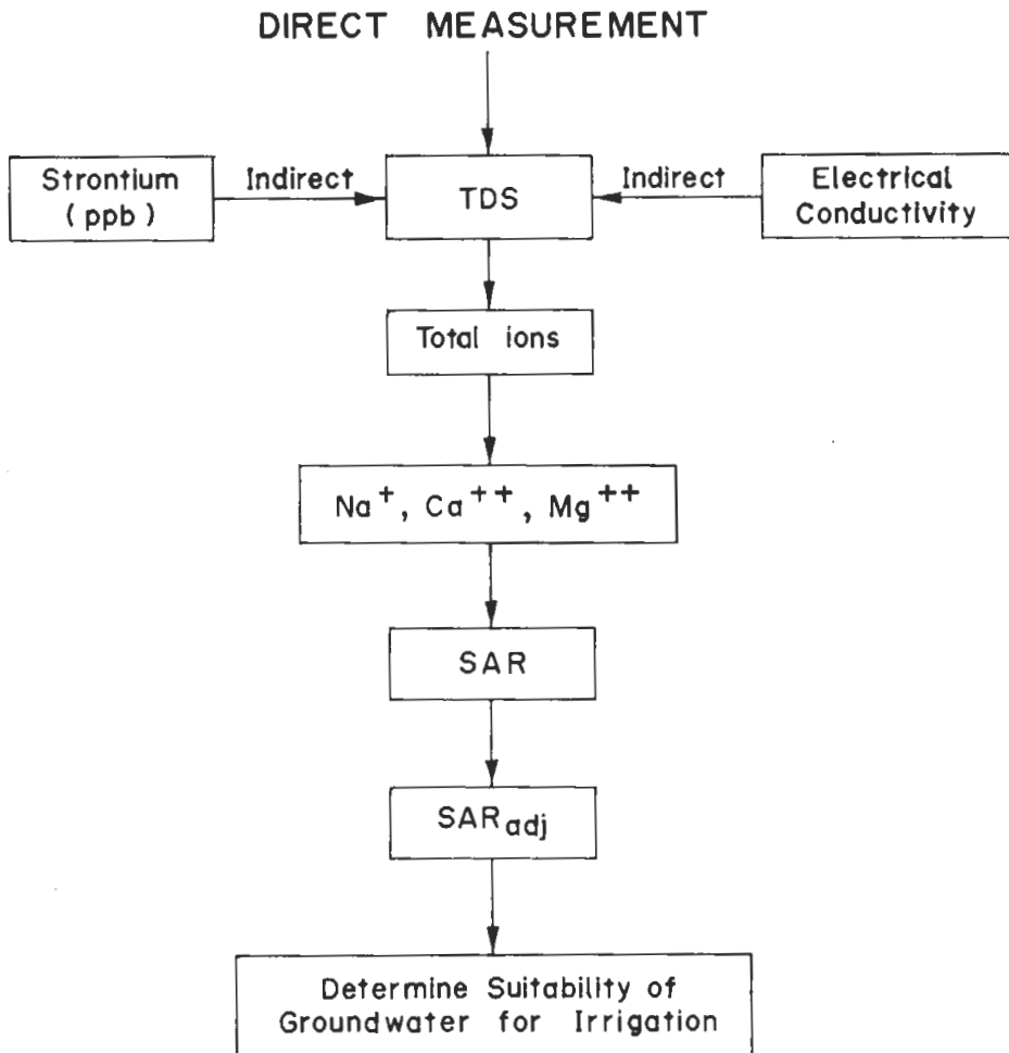
FIG. 8. A systematic approach for calculating SAR_{adj} and determining the suitability of groundwater for irrigation.
