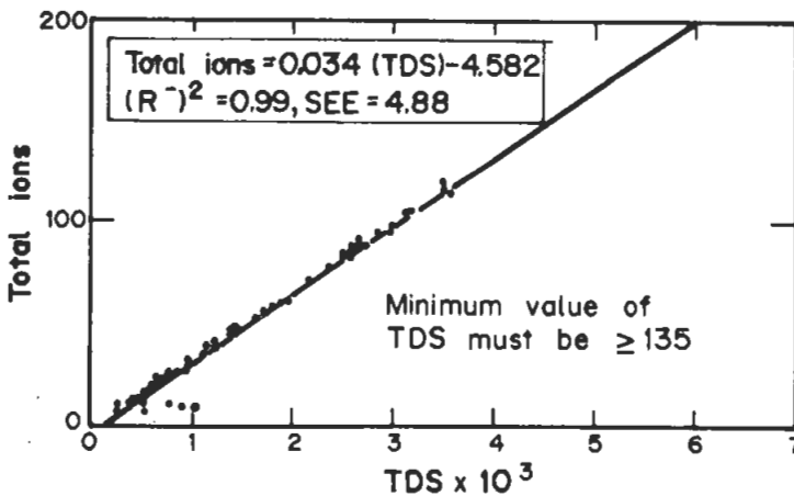
FIG. 2. Relationship of TDS (mg/l) with total ions (meq/l).
