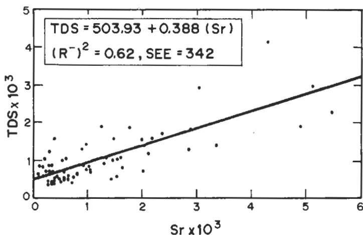
FIG. 7. Relationship of TDS (mg/l) with Strontium (Sr)
