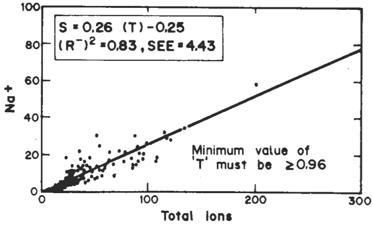
FIG. 3. Relationship of total ions (meq/l) with S (sodium ion) (meq/l).
