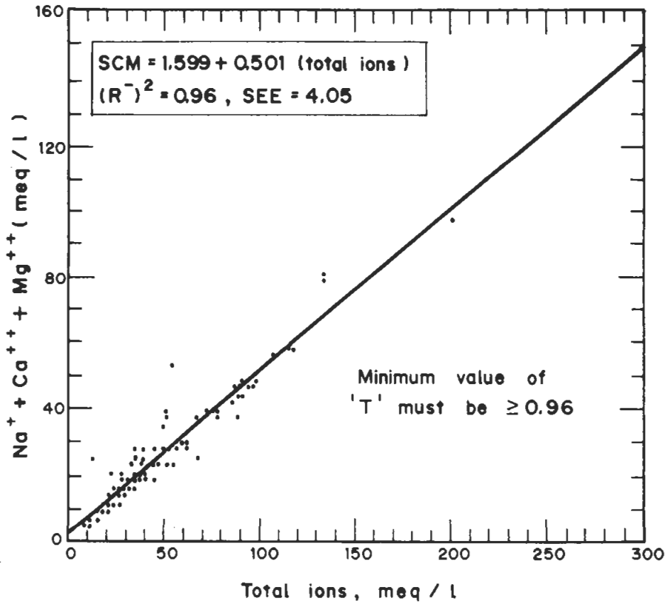
FIG. 4. Relationship of total ions (meq/l) with SCM (Na + , Ca ++ and Mg ++ ).
