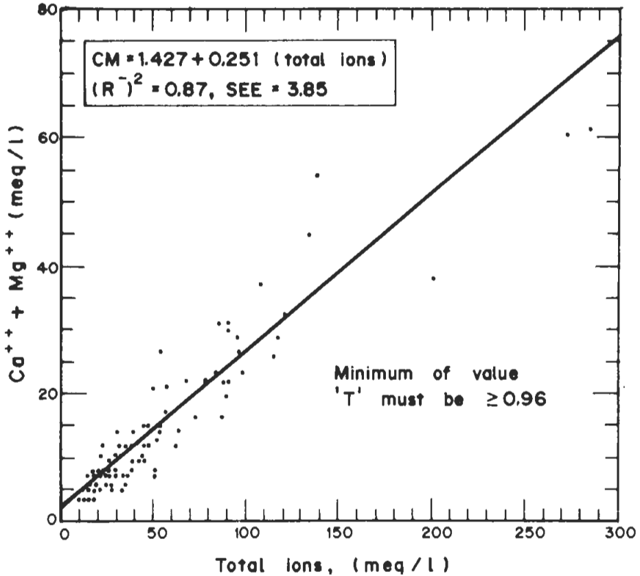
FIG. 5. Relationship of total ions (meq/l) with CM ( \text{Ca}^{++} + \text{Mg}^{++} ).
