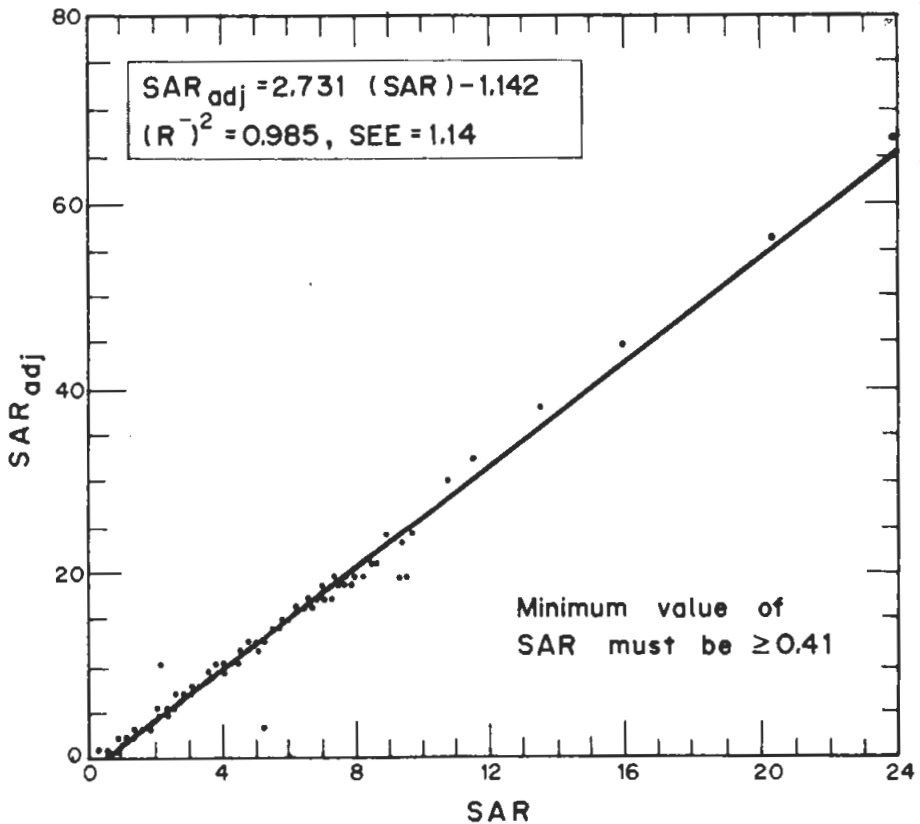
FIG. 6. Relationship of SAR with \text{SAR}_{\text{adj}}
