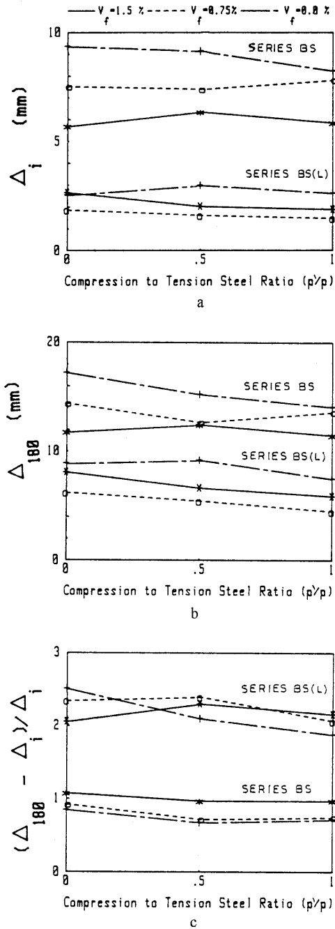
FIG. 7. Effect of p'/p on immediate deflection \Delta_i , long-term deflections at 180 days \Delta_{180} and deflection ratio (\Delta_{180} - \Delta_i) / \Delta_i .
