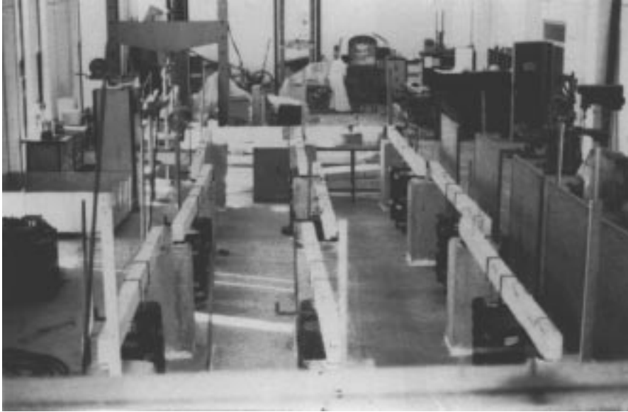
FIG. 2. General view of testing arrangement.
