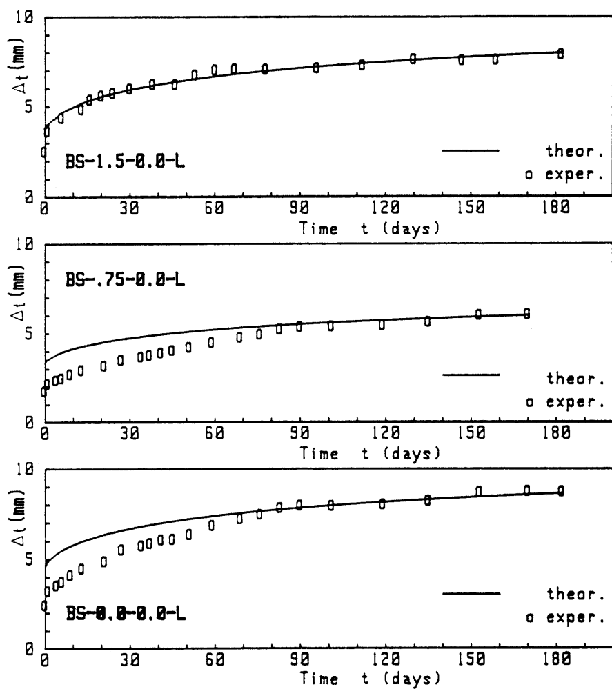
FIG. 11. Comparison of observed and predicted time vs. deflection curves for beams in series BS(L).
