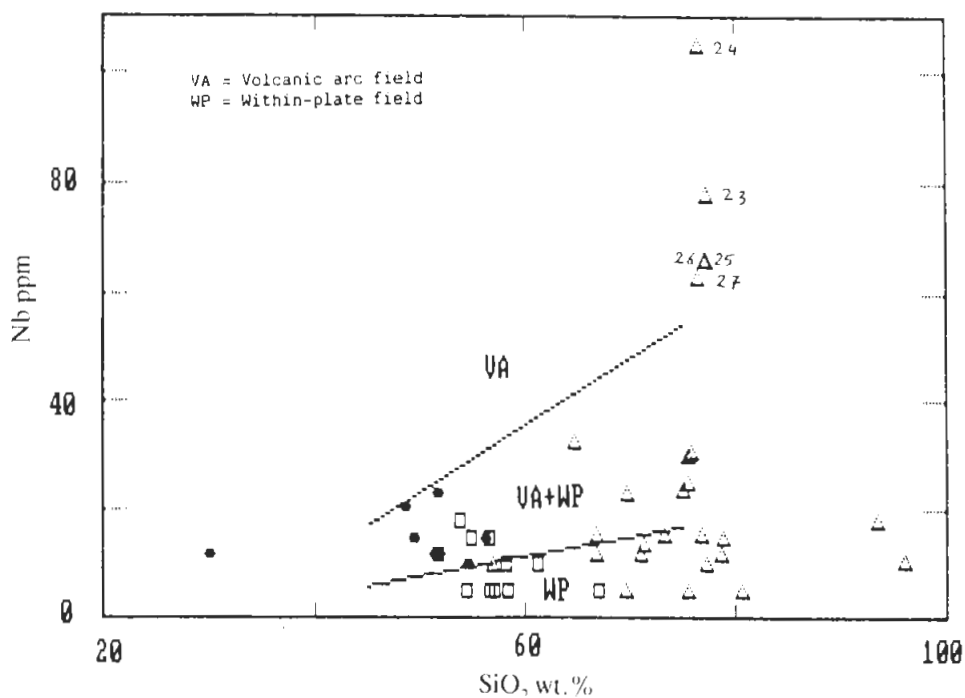
FIG. 9. Nb against SiO 2 diagram for the studied rocks, after Pearce and Gale 1976 (Symbols as in Fig. 5).
