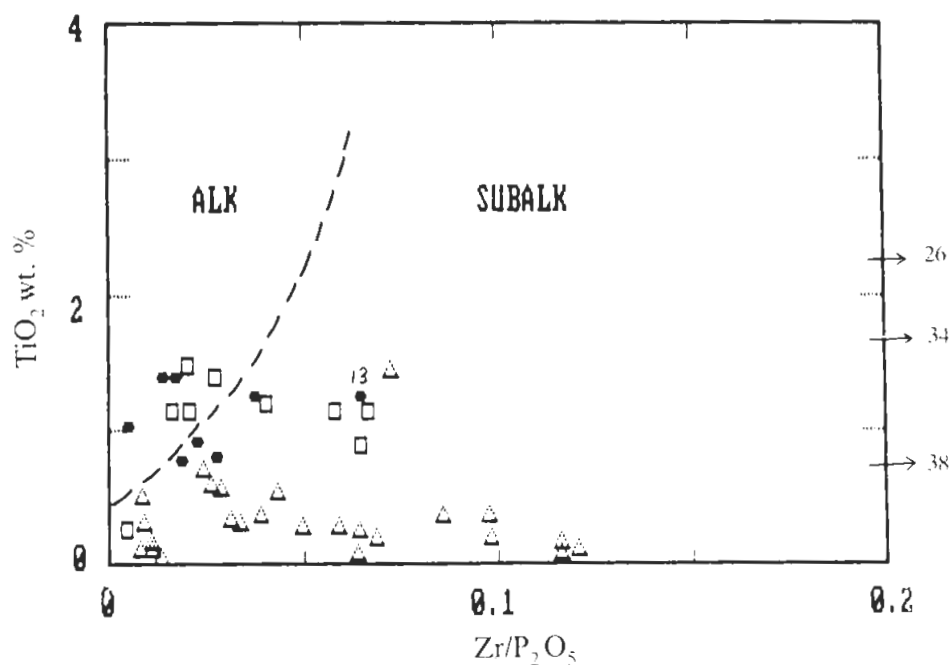
FIG. 6. \text{TiO}_2 against \text{Zr/P}_2\text{O}_5 diagram for the studied rocks, after Winchester and Floyd 1976 (symbols as in Fig. 5).
