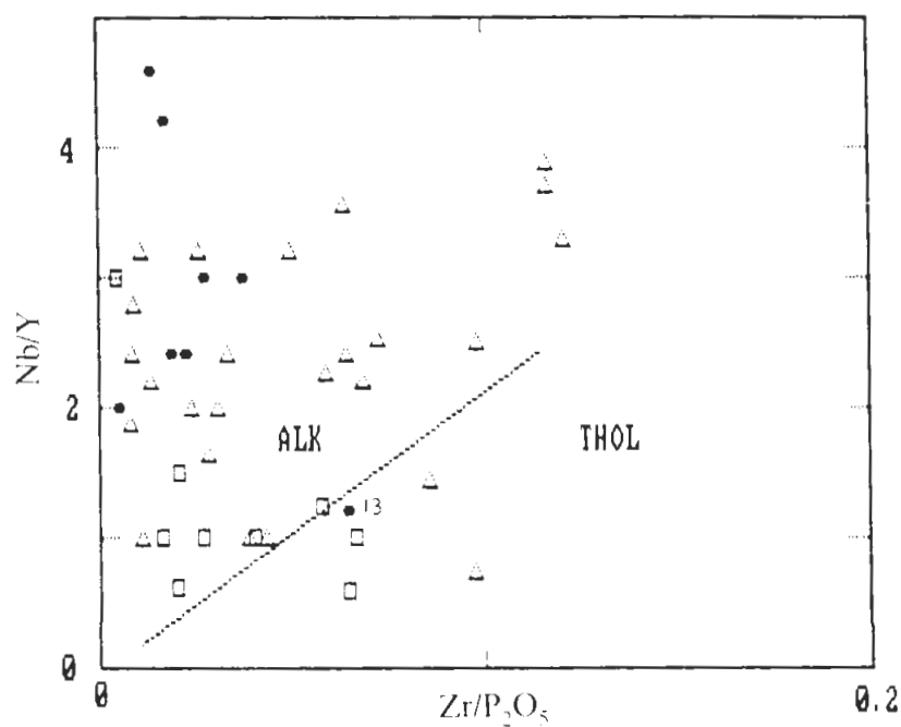
FIG. 7. \text{Nb/Y} against \text{Zr/P}_2\text{O}_5 diagram for the studied rocks, after Winchester and Floyd 1976 (symbols as in Fig. 5).
