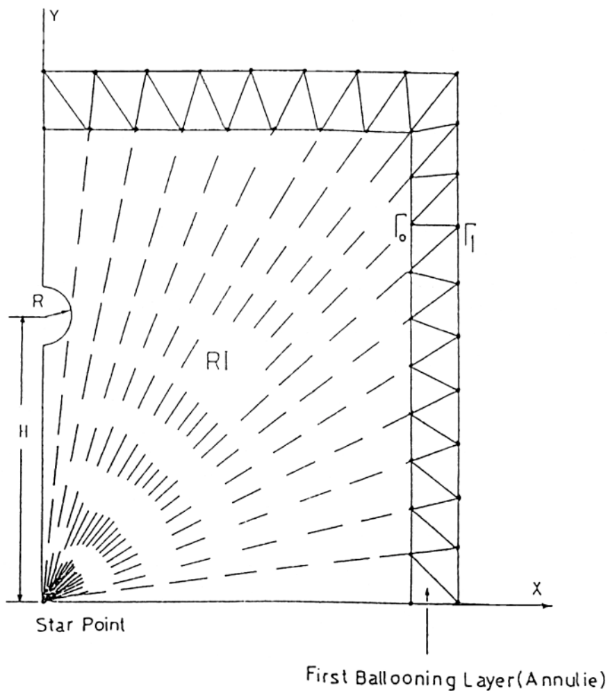
FIG. 3. The conductor-to-plane FE grid is bounded exterior region for the application of the ballooning technique.
