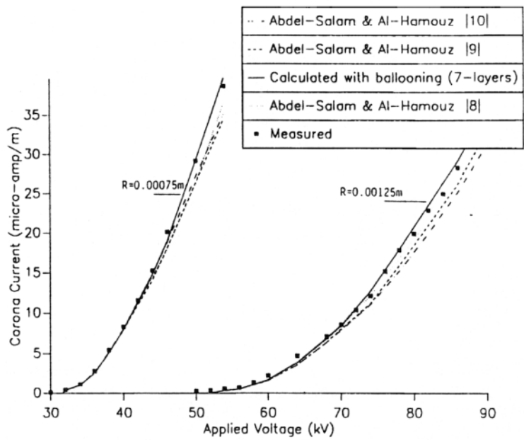
FIG. 9. Calculated and measured V-I characteristics of laboratory transmission-line configurations ( H = 0.29\text{ m} , \eta = 1 ).
