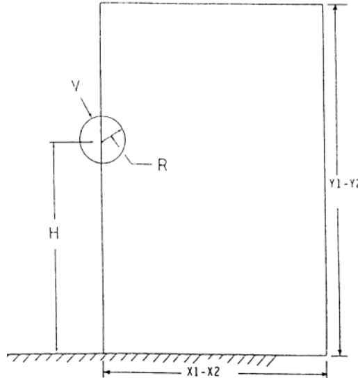
FIG. 1. Conductor-to-plane configuration.
