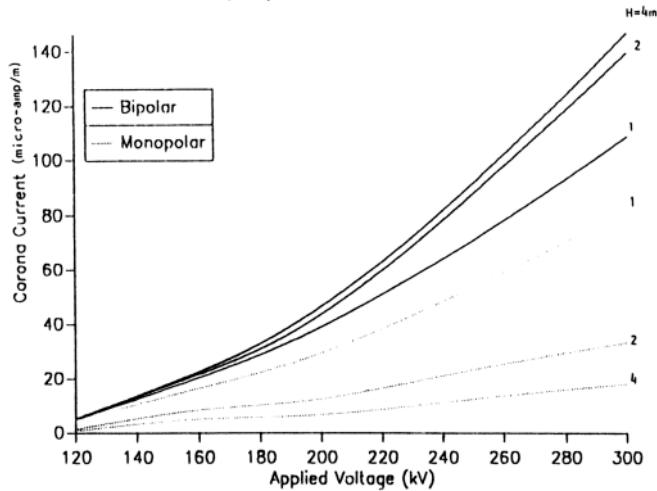
Figure 8. Effect of the conductor's height on the monopolar and bipolar components of the corona current ( D = 3 m, R = 0.0025 m, \eta = 1 ).
