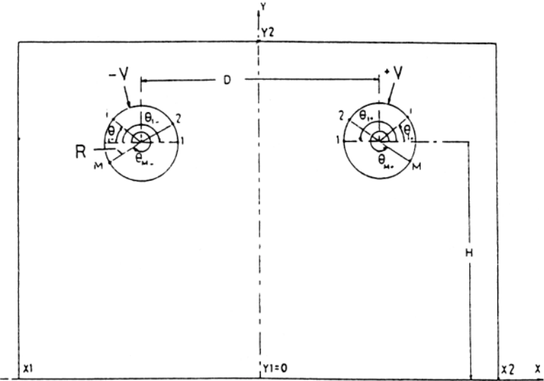
Figure 1. Region where the field lines and equipotential contours are mapped, \theta_i defines the angle at which the i^{th} field line emanates.
