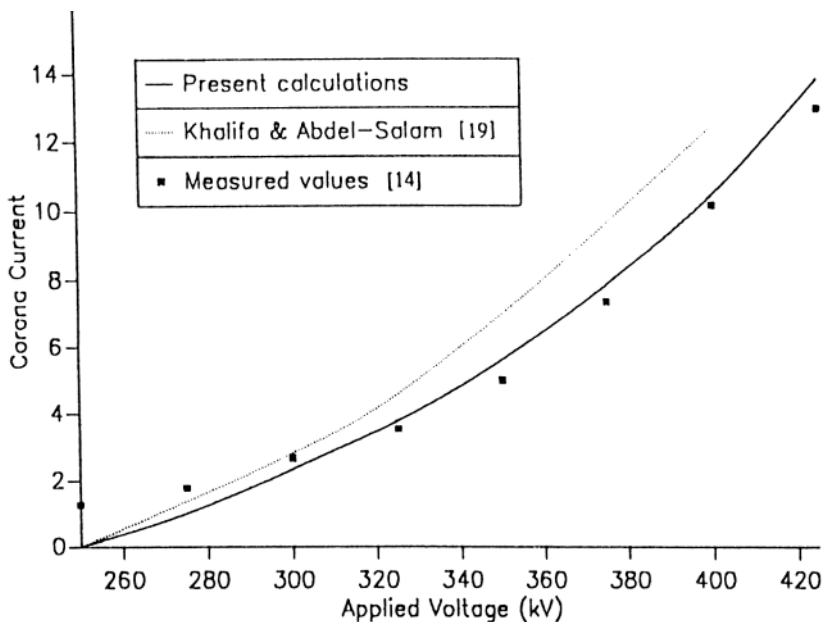
Figure 10. Calculated V-I characteristics of a full-scale bipolar transmission line configuration as compared to previous measured and calculated values ( H = 9.15 m, D = 10.36 m, R = 0.0102 m, \eta = 0.7 ).
