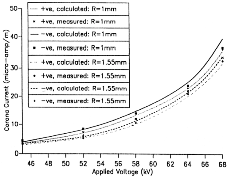
Figure 9. Effect of the conductor's radii on the positive and negative V-I characteristics measured and calculated by the proposed method for a bipolar transmission line configuration ( H = 0.295 m, D = 0.45 m, \eta = 1 ).
