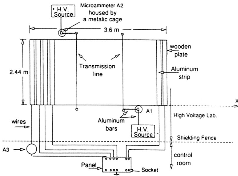
Figure 4. Experimental set-up: (a) plan-view.
