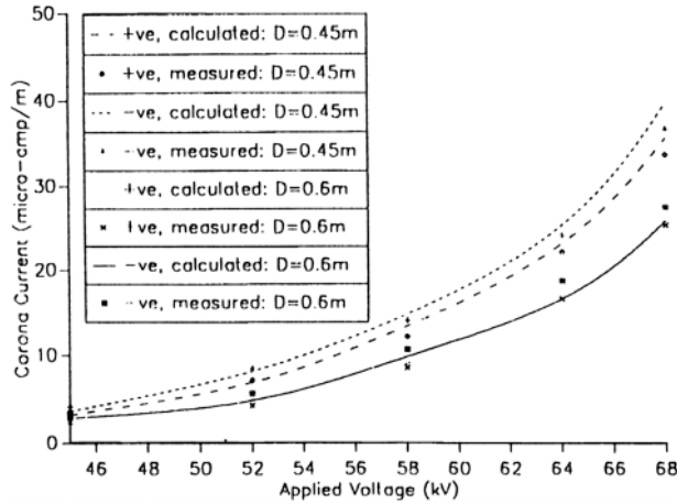
Figure 7. Effect of the conductor's spacing on the positive and negative, V-I characteristics measured and calculated by the proposed method for a bipolar transmission line configuration ( R = 0.001 m, H = 0.295 m, \eta = 1 ).
