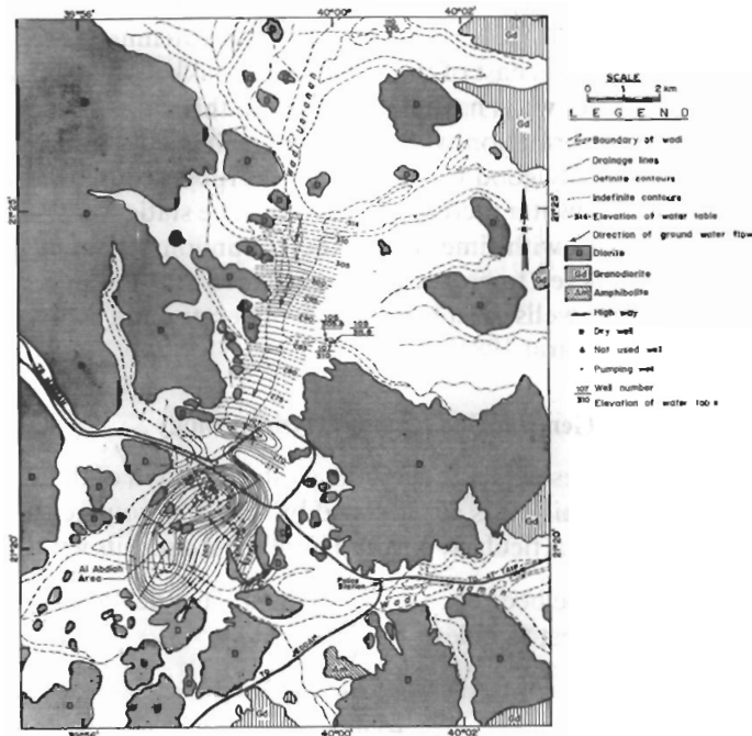
FIG. 2. Groundwater table map of Wadi Uoranah-Al-Abdiah area.
