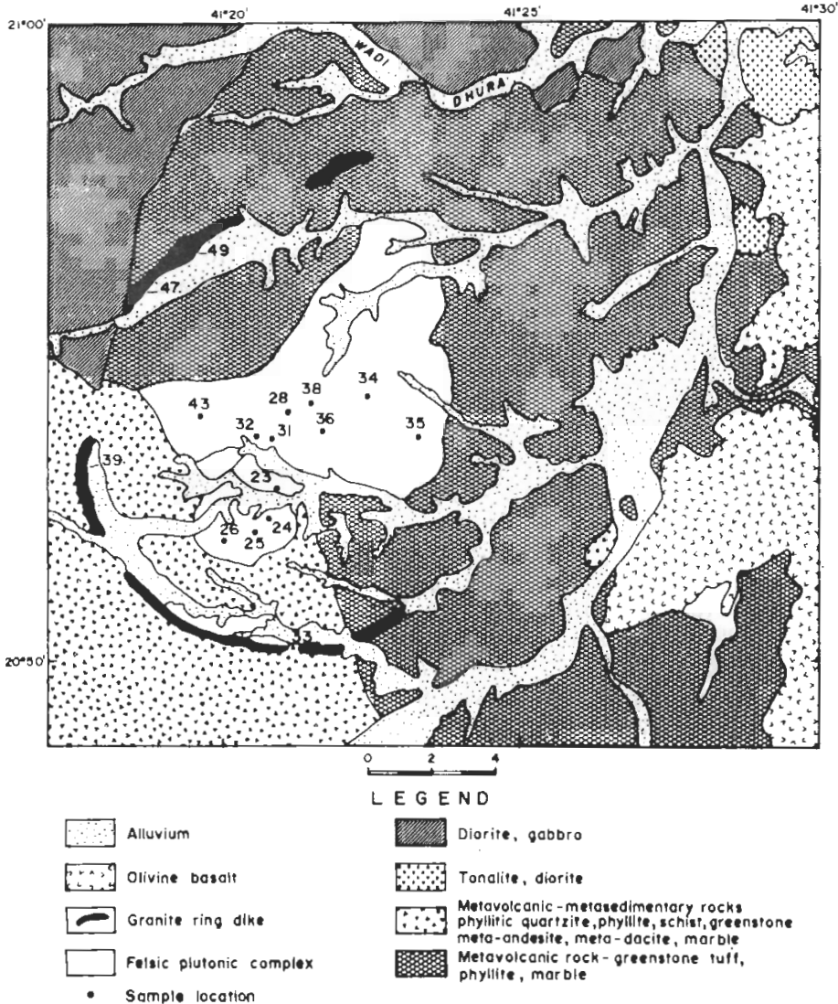
FIG. 3. Simplified geological map of the Wadi Turabah ring complex (after Greene and Gonzalez 1980).
