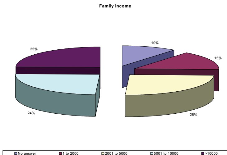
Fig. 3. Family income.
