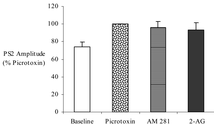
Fig. 5. The CB 1 receptor antagonist AM281 ( 500\text{nM} and striped bar) totally blocked the effect of subsequently perfused 2-AG ( 10 \mu\text{M} and black bar), in slices where epileptiform activity had been induced by perfusion of picrotoxin ( 500\text{nM} and dotted bar). Data are presented as mean amplitude ( p<0.05 , n=7 ).
