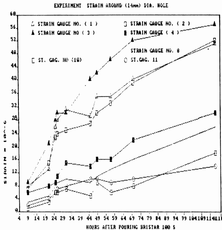
FIG. 5. Strain-time graphs for some of the strain gauge for experiment 2 (a).
