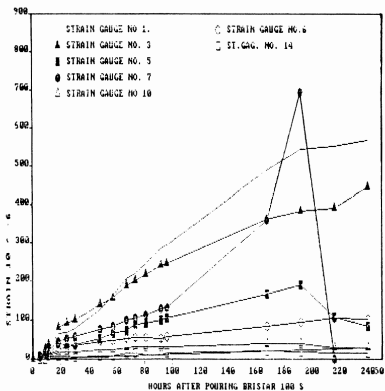
FIG. 3. Time strain graph for some of the strain gauges for Experiment No. 1.
