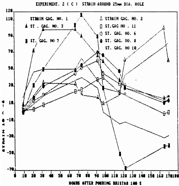
FIG. 7. Strain-time graph for some of the strain gauges for Experiment No. 2(c).
