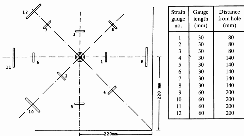
FIG. 4. Positioning of strain-gauges for experiment no. 2 (a, b and c).
