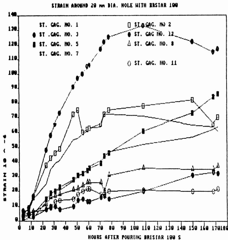
FIG. 6. Strain-time graph for some of strain gauges for Experiment 2(b).
