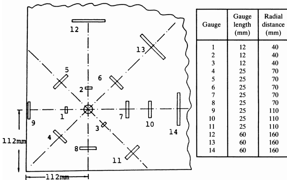
FIG. 2. Positioning of strain gauges around 14 mm dia. borehole.
