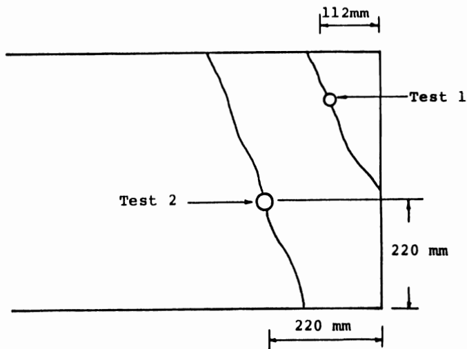
FIG. 8. Experiment 2(c); extension of crack to other side of the hole after 70 hours.
