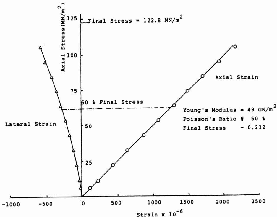
FIG. 1. Stress-strain relationship for specimen no. 2.
