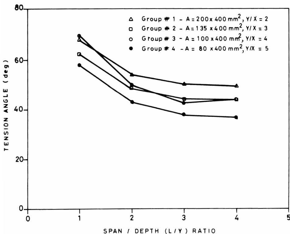
FIG. 5. Effect of span/depth ( L/Y ) ratio on the tension crack angle.
