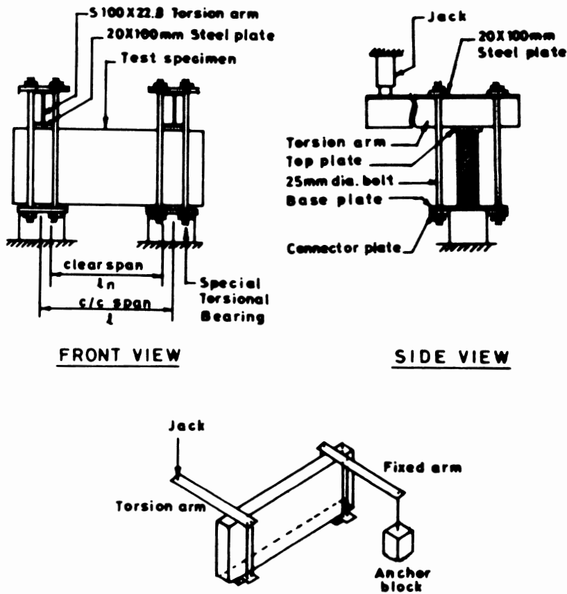
FIG. 1. Test set-up.
