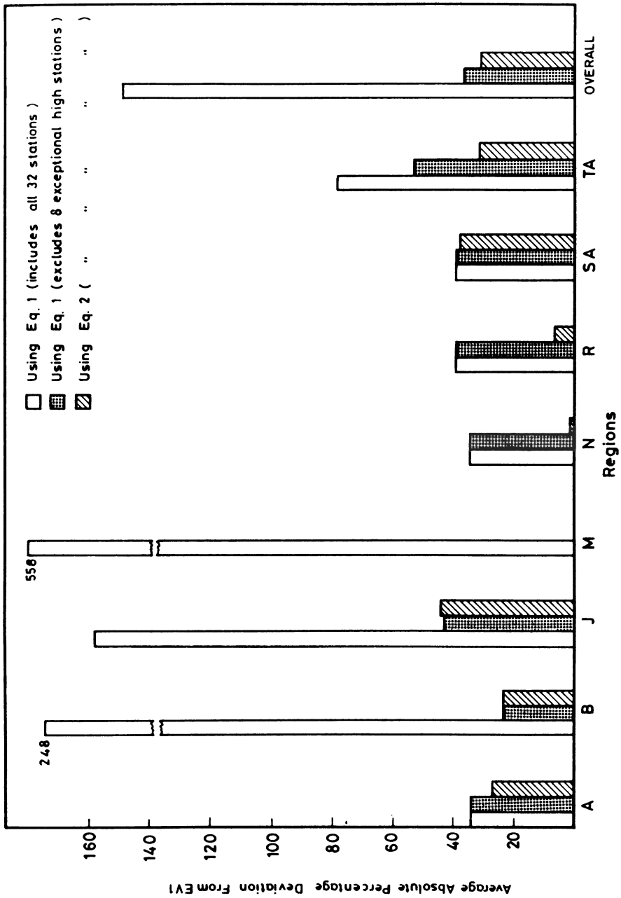
FIG. 2. Absolute percentage deviation from EV1 (T = 25 years).
