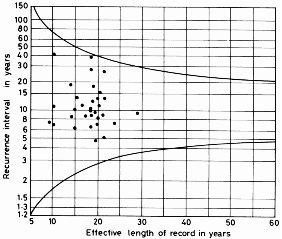
FIG. 1. Homogeneity test graph.
