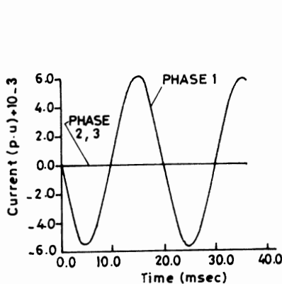
FIG. 5(a). Current waveform for finite source.
