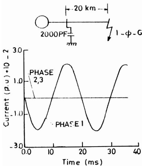
FIG. 7(a). Current waveform.
