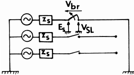
FIG. 3(a). Last pole-to-clear.
