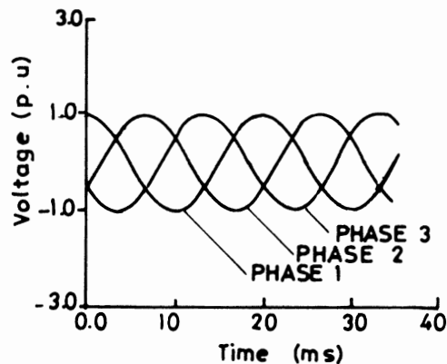
FIG. 7(b). Voltage waveform.
