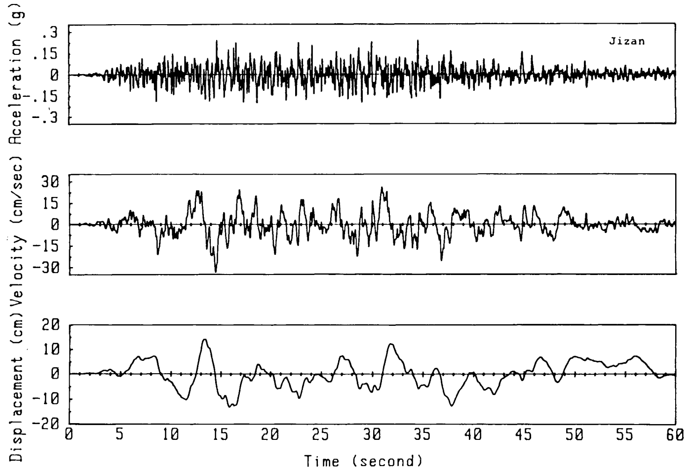
FIG. 3. Time history of ground motion for Jizan.
