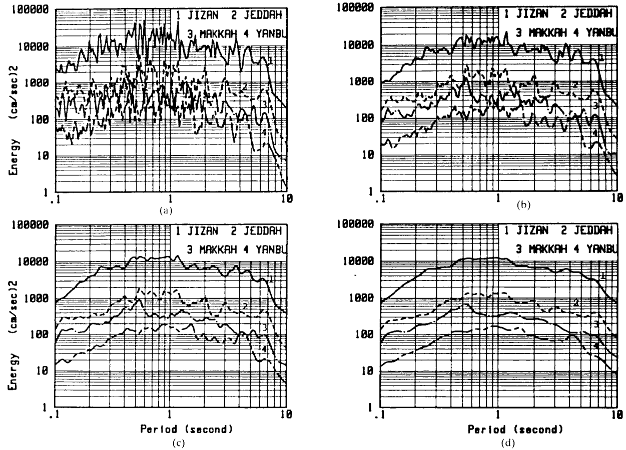
FIG. 8. Energy input per unit mass spectra: (a) 0% damping, (b) 2% damping, (c) 5% damping, (d) 10% damping.
