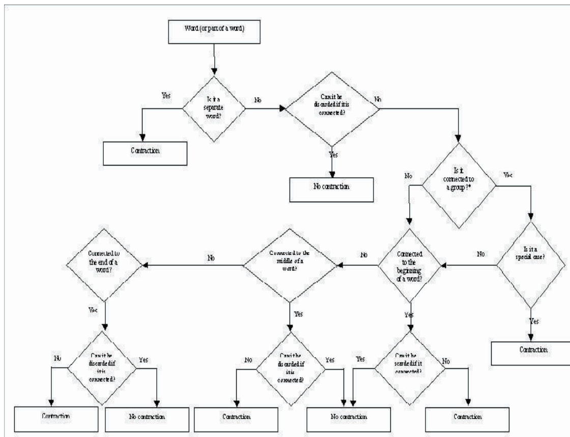
Fig. 7. Translation rules.
