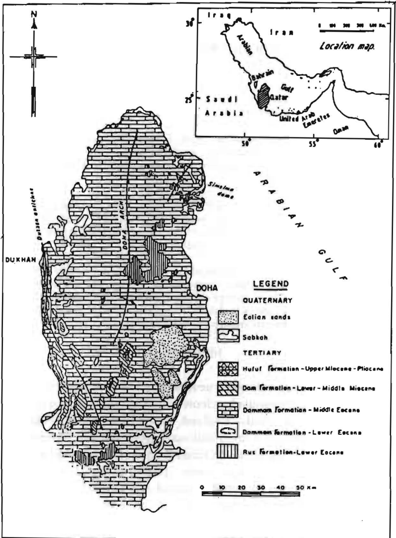
Fig. 1. Geological map of Qatar Peninsula
