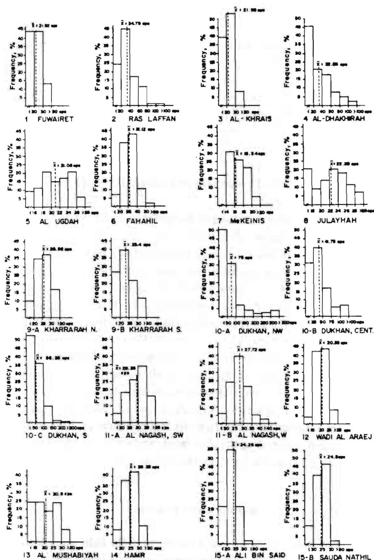
Fig. 3. Histograms of radioactivity in the anomalous localities
