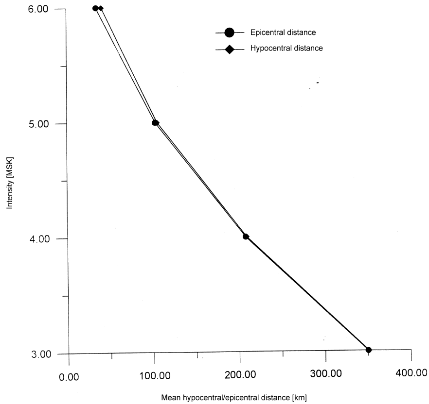
Fig. 5. Intensity-mean distance graph of October 12m 1992 earchquake in Egypt.
