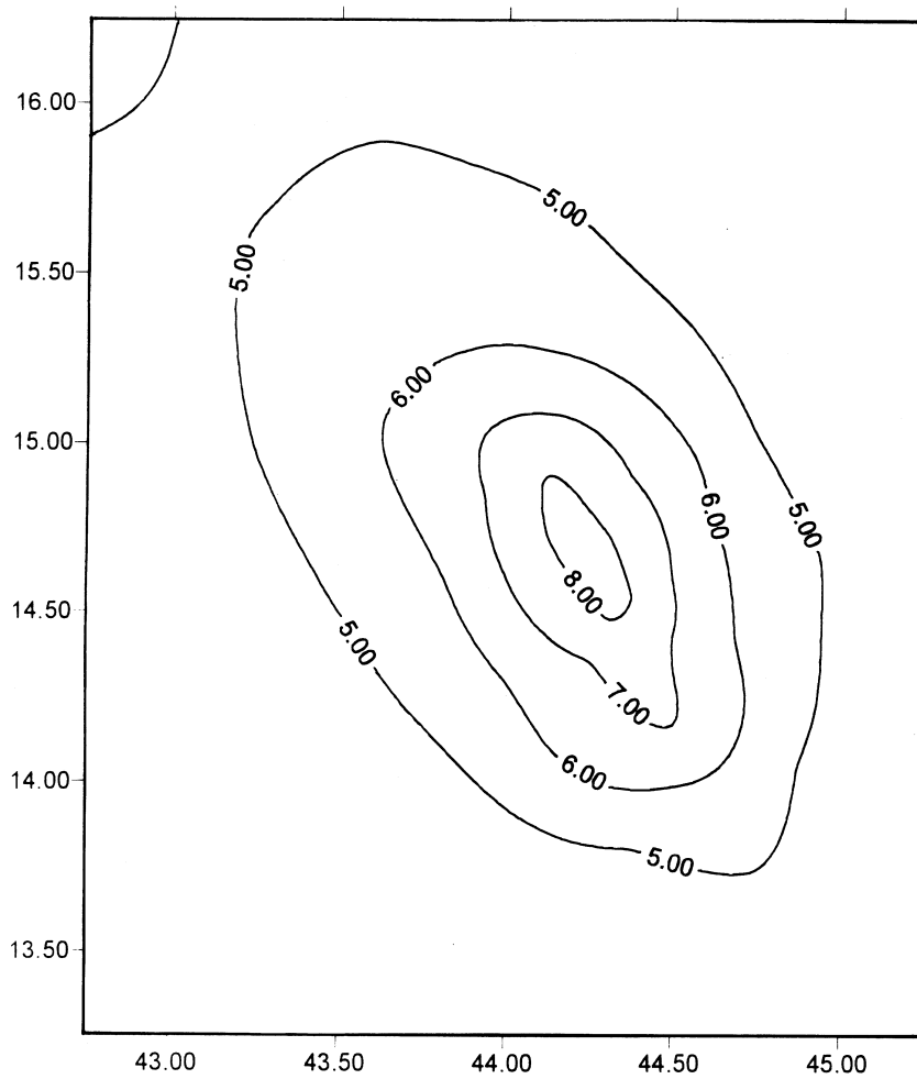
Fig. 3. Computerized isoseismal map of December 13, 1982 earthquake in Dhamar, Yemen. Macroseismic epicenter 14.68 N; 44.24 E. Reference Shehata et al. (1983). Isoseismal lines are based on MSK intensity scale.
